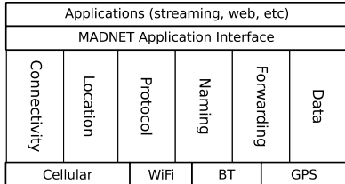
Figure 1. MADNet Architecture
