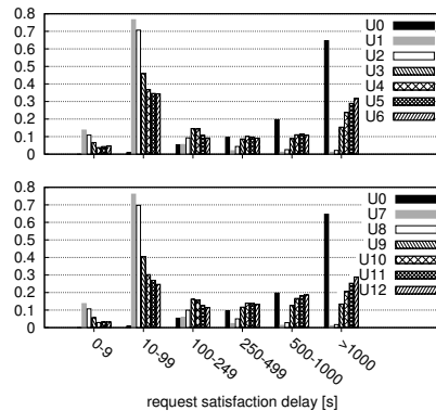
Figure 10. Request satisfaction delay distribution of upload requests
