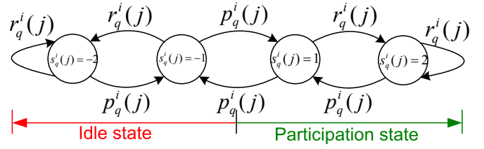
Fig. 3. An example of the Gur Game with associated memory size M = 2 , where positive number states give the corresponding output of “participation” and negative numbers state represent “idle” decision.
