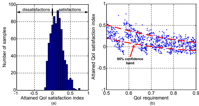
Fig. 9. The received QoI satisfaction index: (a) the histogram and (b) w.r.t. different required QoI levels.
